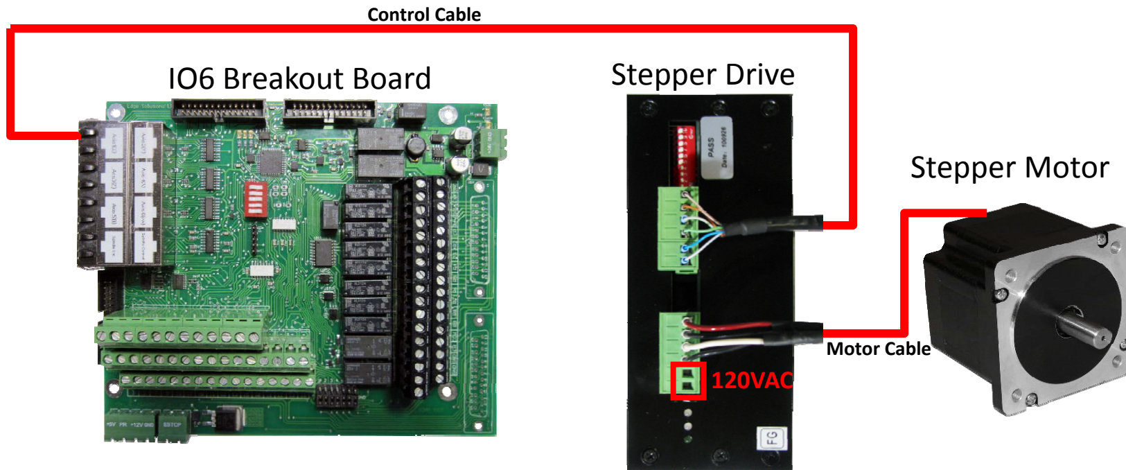
Control Connector
